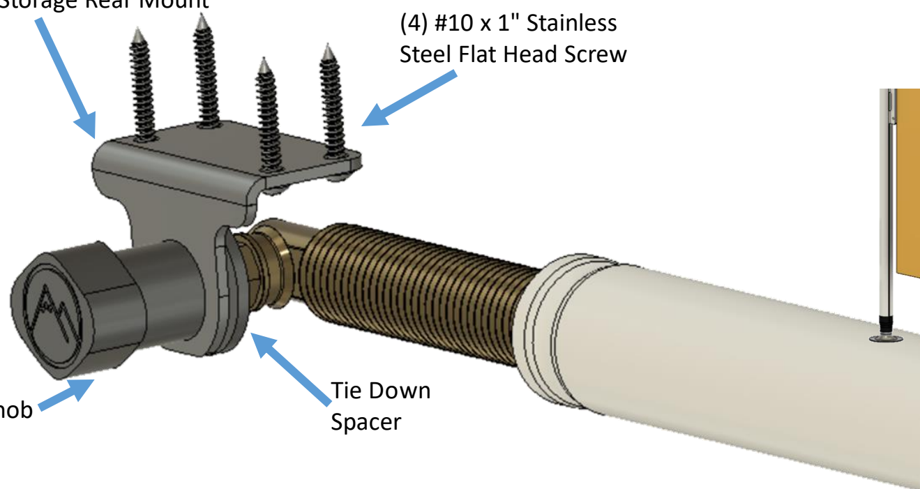
Side Storage Rear Mount
